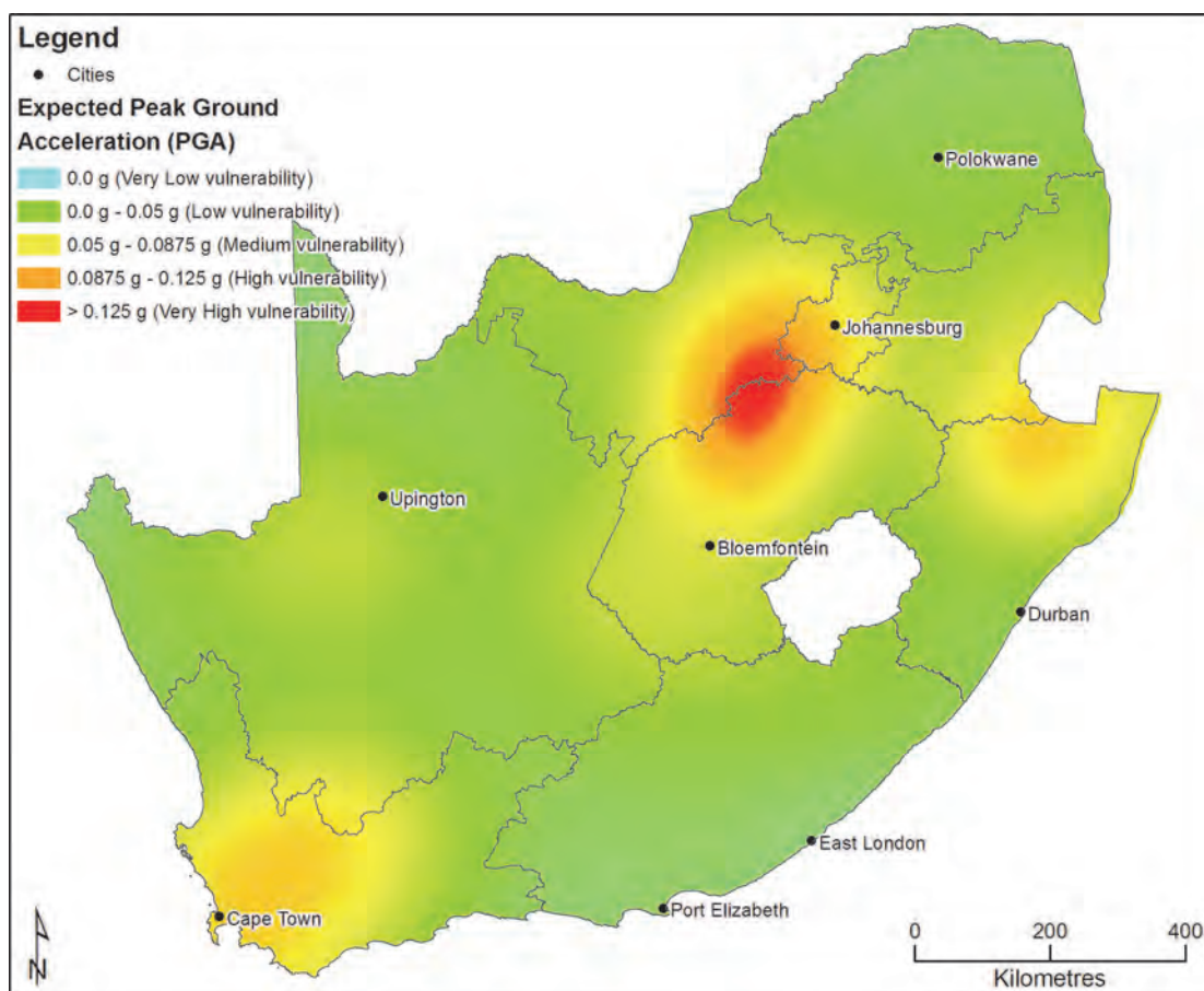
Figure 22: Map of current seismic vulnerability (hazard) for South Africa. This map shows the expected PGA with a 10% probability of being exceeded at least once in a 50 year period.
