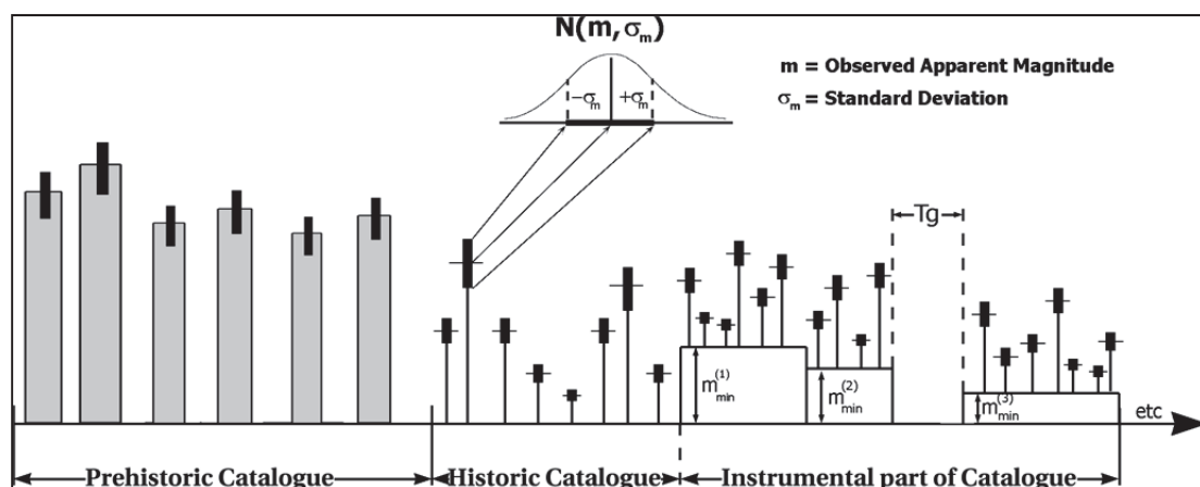
Figure 21: Illustration of data which can be used to obtain recurrence parameters for the specified seismic source (Modified after Kijko and Sellevoll, 1992)
