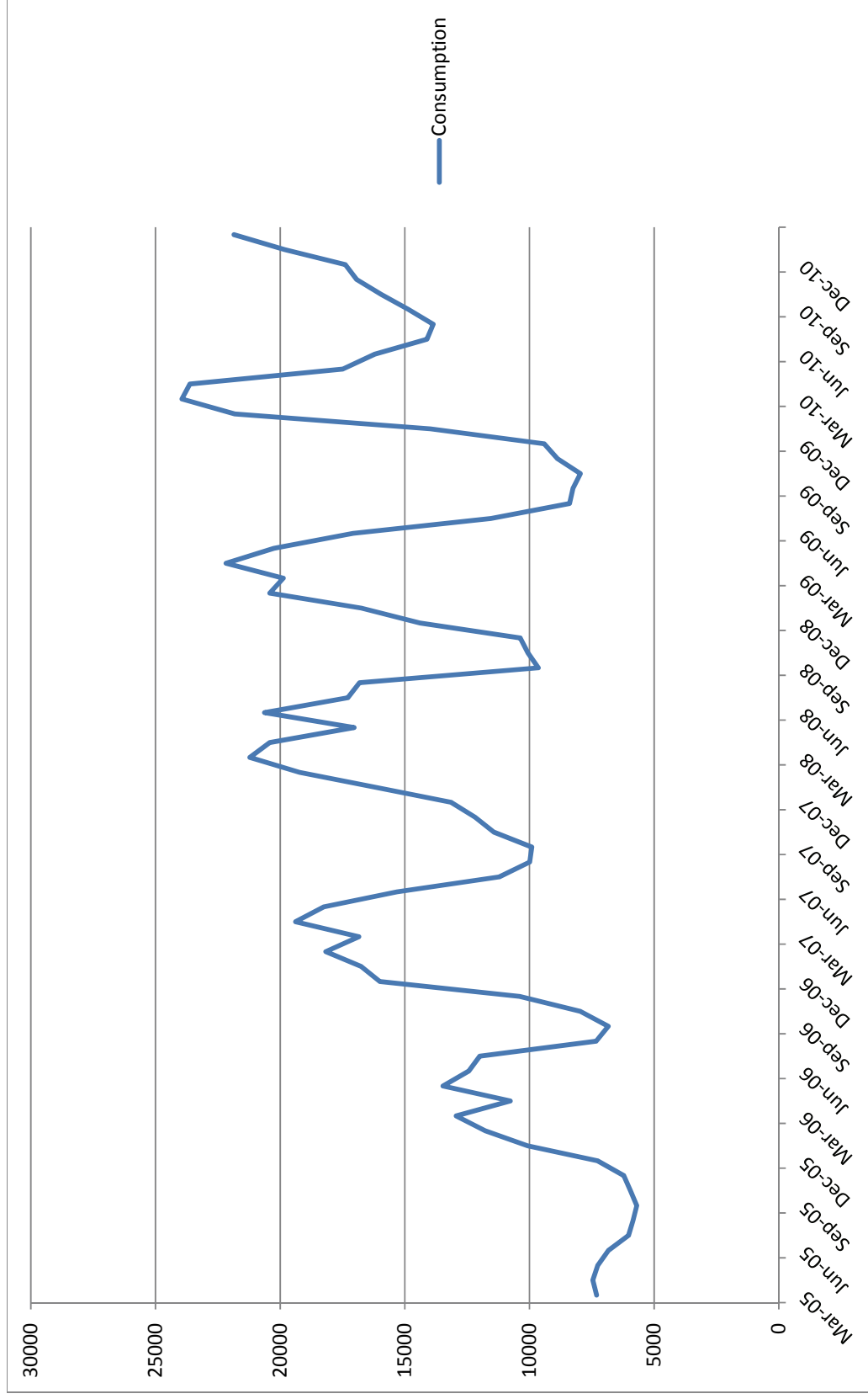
Figure 27: Farmland Water Consumption, March 2005 to February 2011. [Smoothed]
